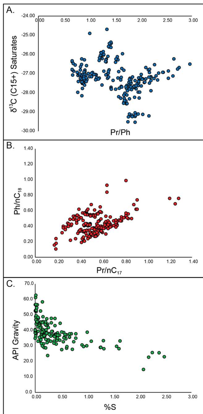
Figure 10. Bivariate cross-plots of the Upper Cretaceous Eagled Ford sourced oils identified in GeoMark's OILS database. In addition to the organofacies variation in the Eagled Ford Shale itself, there is also significant thermal maturity variations across the play and potential for mixing with self-sourced fluids in the various reservoirs of the Eagle Ford. All of these factors play a role in the wide range of geochemical signatures across the play. (A) Carbon isotope signatures ( \delta^{13}\text{C}_{\text{VPDB}} ) of the C15+ saturate relative to Pr/Ph ratio. (B) Pr/nC 17 relative to Ph/nC 18 . (C) API gravity (60 °F) relative to weight % sulfur.
